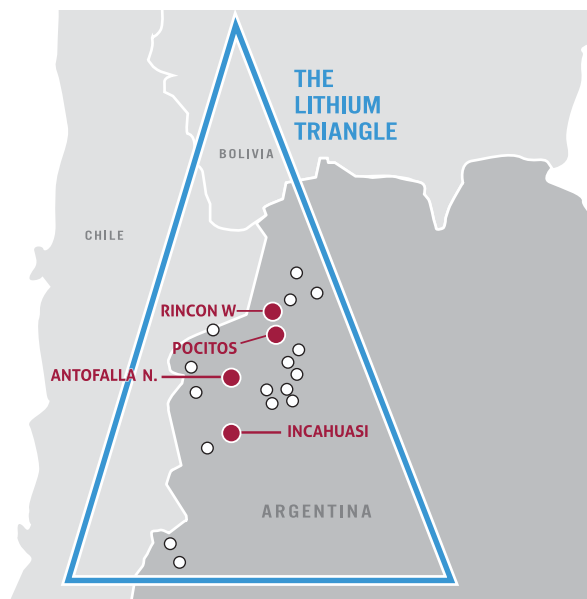
● Argentina Lithium Projects ○ Other Lithium Projects
