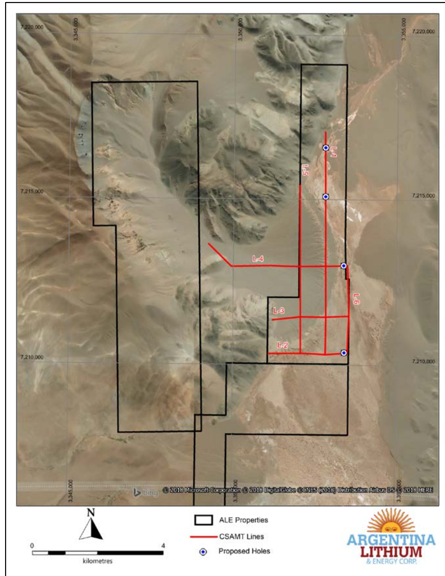
Figure 1. Antofalla Norte CSAMT Survey lines and Proposed Drill Holes
