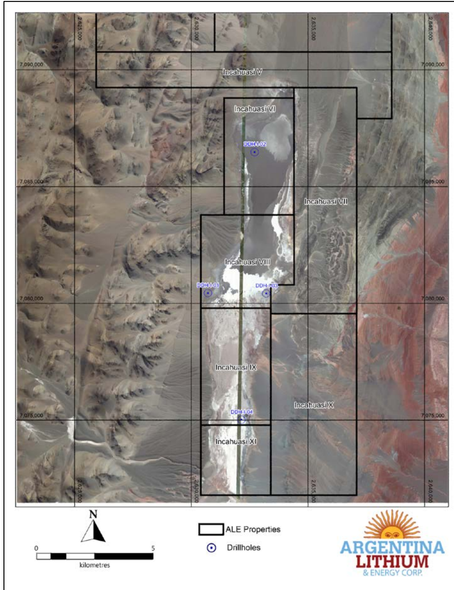
Figure 3. Incahuasi Drill Hole locations
